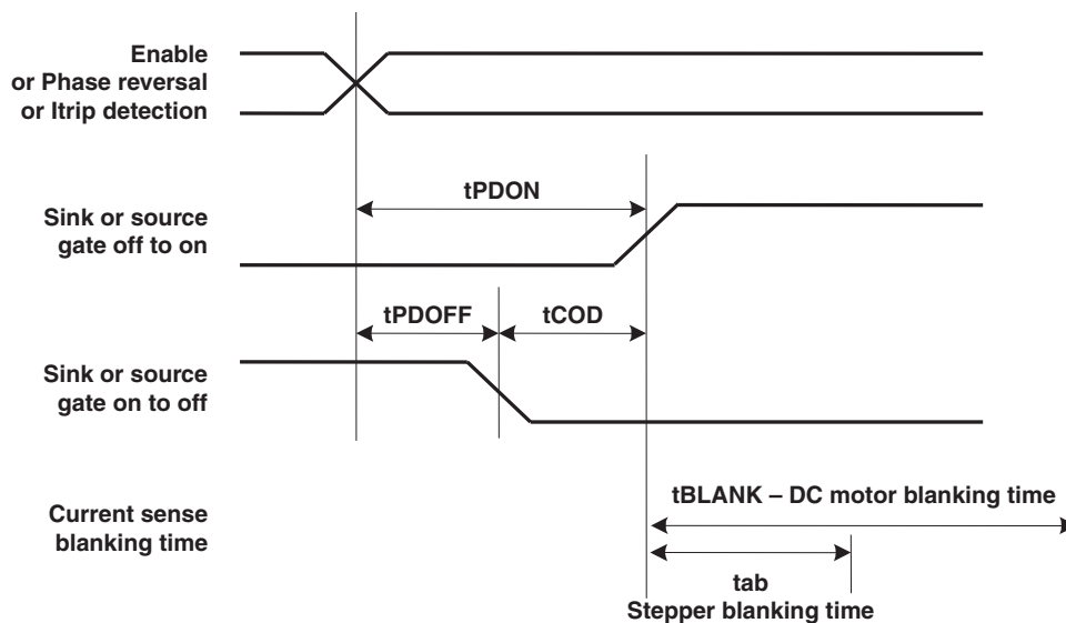
Figure 17. Crossover and Blanking Timing for H-Bridge
