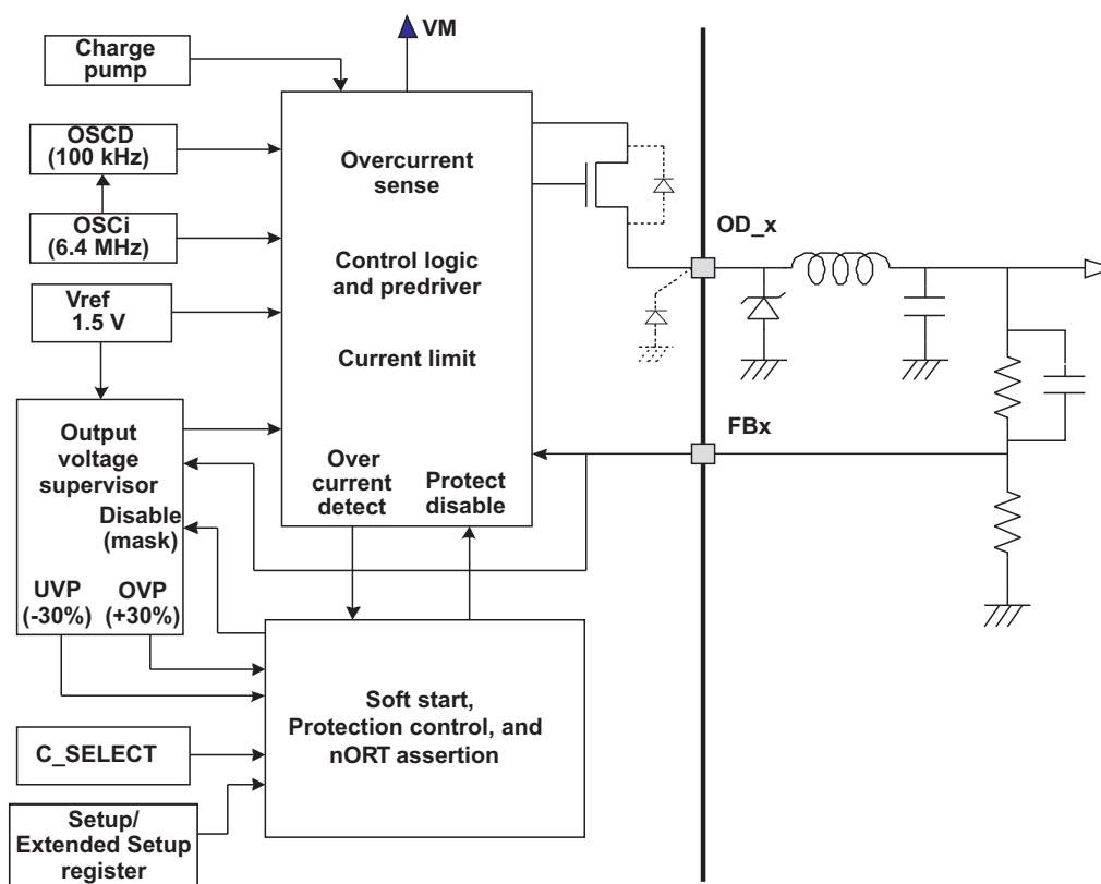
Figure 21. DC-DC Converter
